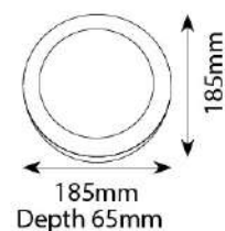
Product Code : UL 131 Material : Aluminium Die Casting + PC Diffuser LED : 12W Edison LED with Philips Driver Color Temperature : 3000K/6000K Finish : Graphite Grey IP Rating: IP 54
