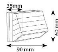
Product Code : UL 110 Material : Aluminium Die Casting + PC Diffuser LED : 4W Edison LED Color Temperature : 3000K Finish : Graphite Grey IP Rating: IP 54
