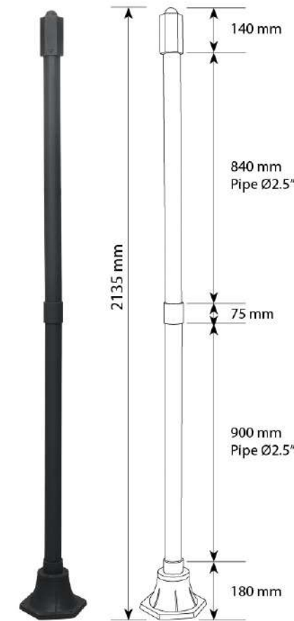
Product Code : P47 Pole Material : Aluminium Casting & Extrusion Base Dia : Ø250 mm
