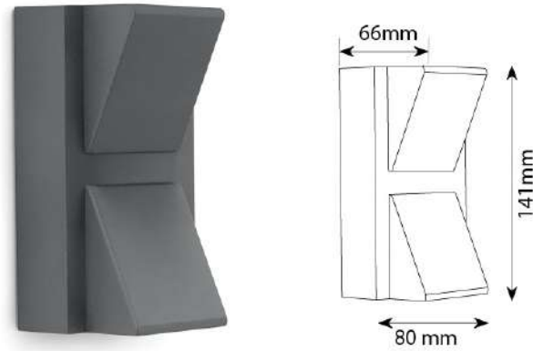
Product Code : UL 8091-2 Material : Aluminium Die Casting + Glass LED : 2 x 3W Edison/ Everlight LED Color Temperature : 3000K Finish : Graphite Grey IP Rating: IP 54
