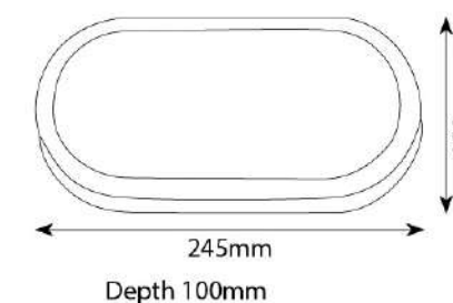
Product Code : UL 136 Material : Aluminium Die Casting & ABS + PC Diffuser LED : 12W Edison LED Color Temperature : 3000K/6000K Finish : Graphite Grey IP Rating: IP 54
