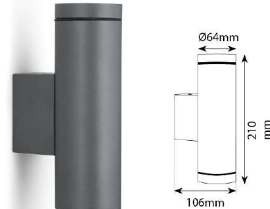
Product Code : UL 299 Material : Aluminium Extrusion & Casting + Glass Finish : Graphite Grey Holder: 2 x GU10 | IP Rating: IP 54
