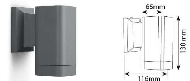
Product Code : UL 301 Material : Aluminium Extrusion & Casting + Glass Finish : Graphite Grey Holder: GU10 | IP Rating: IP 54
