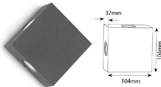
Product Code : UL 109 Material : Aluminium Die Casting + Glass LED : 4 x 1W Cree LED Color Temperature : 3000K Finish : Graphite Grey IP Rating: IP 54
