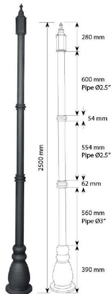
Product Code : P23 Pole Material : Aluminium Casting & Extrusion Base Dia : Ø260 mm
