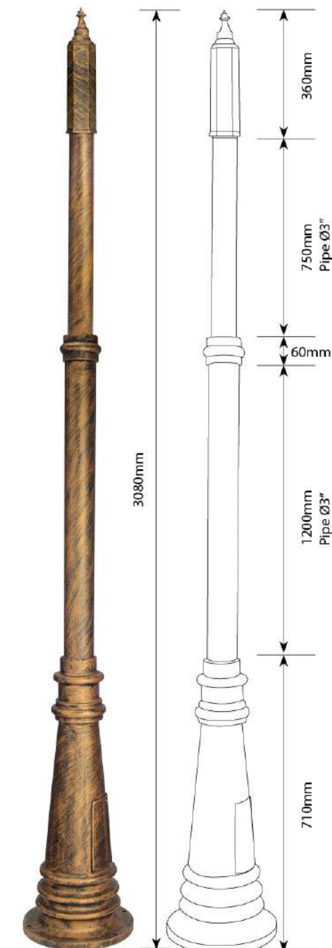
Product Code : P27 Pole Material : Aluminium Casting & Extrusion Base Dia : Ø290 mm
