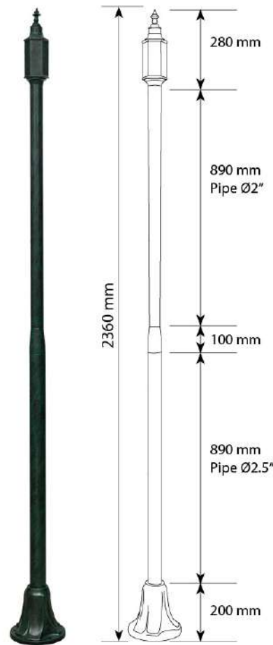
Product Code : P17 Pole Material : Aluminium Casting & Extrusion Base Dia : Ø210 mm
