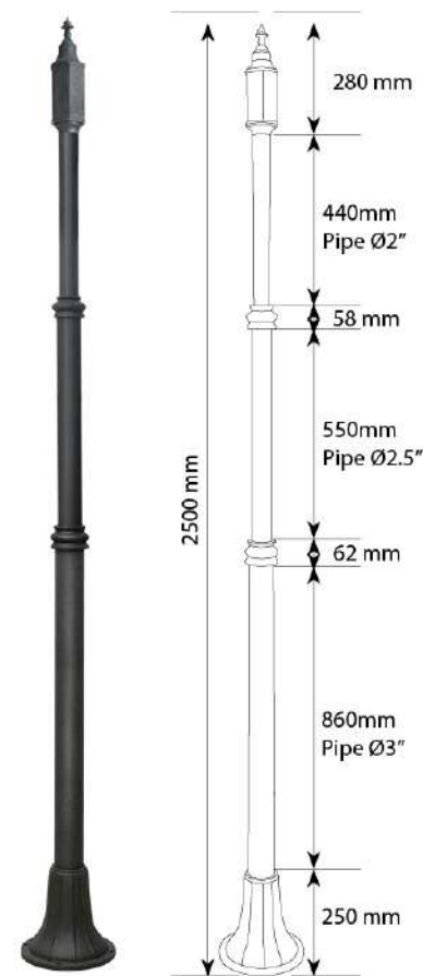
Product Code : P21 Pole Material : Aluminium Casting & Extrusion Base Dia : Ø240 mm
