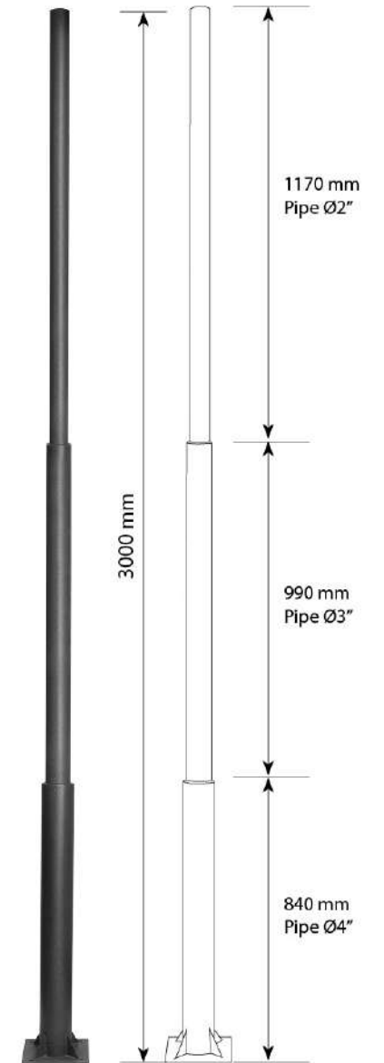
Product Code : 234 Pole Material : MS Base Dia : 250 mm x 250 mm
