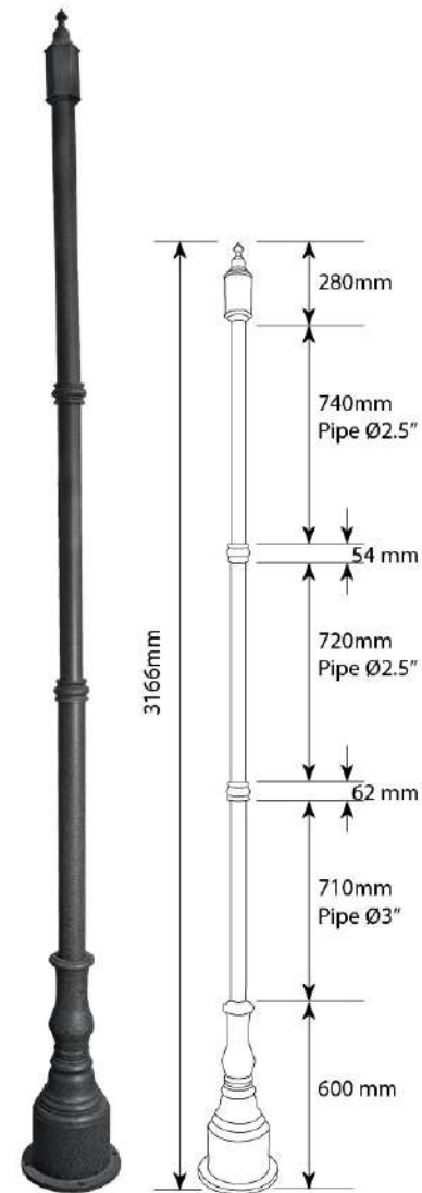
Product Code : P25 Pole Material : Aluminium Casting & Extrusion Base Dia : Ø275 mm
