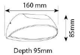
Product Code : UL 115 Material : Aluminium Die Casting + PC Diffuser LED : 12W Edison LED Color Temperature : 3000K/6000K Finish : Graphite Grey IP Rating: IP 54
