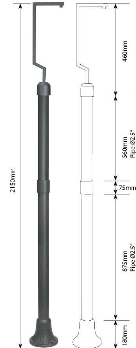
Product Code : P7 Pole Material : Aluminium Casting & Extrusion Base Dia : Ø210 mm
