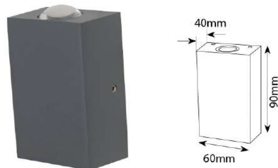
Product Code : UL 108 Material : Aluminium Die Casting + Glass LED : 2 x 1W Cree LED Color Temperature : 3000K Finish : Graphite Grey IP Rating: IP 54
