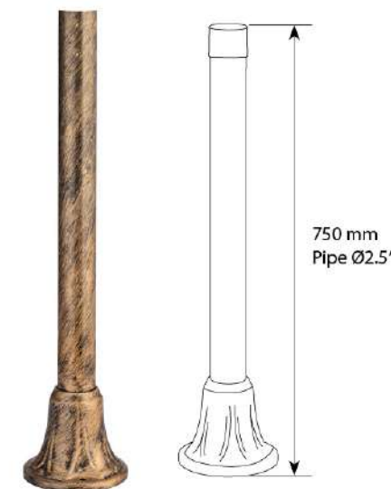
Product Code : P3 Pole Material : Aluminium Casting & Extrusion Base Dia : Ø170 mm
