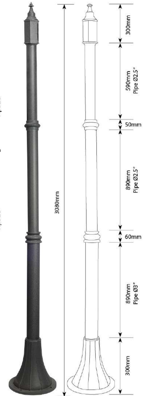
Product Code : P22 Pole Material : Aluminium Casting & Extrusion Base Dia : Ø290 mm
