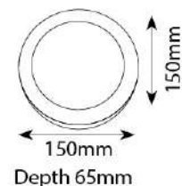
Product Code : UL 127 Material : Aluminium Die Casting + PC Diffuser LED : 6W Edison LED with Philips Driver Color Temperature : 3000K/6000K Finish : Graphite Grey IP Rating: IP 54
