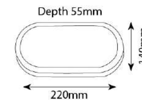
Product Code : UL 122 Material : Aluminium Die Casting + PC Diffuser LED : 12W Edison LED with Philips Driver Color Temperature : 3000K/6000K Finish : Graphite Grey IP Rating: IP 54
