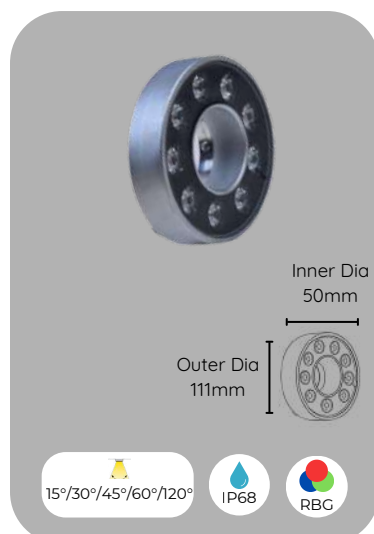
18W Nozzle Pass Fountain Light (12V)
