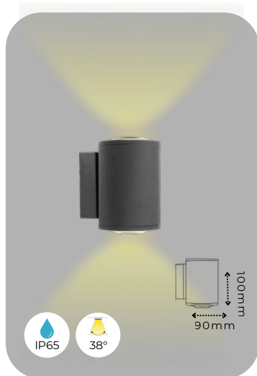
12W Brick 6X2
