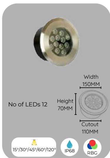
24W AX SP CC (12V)
